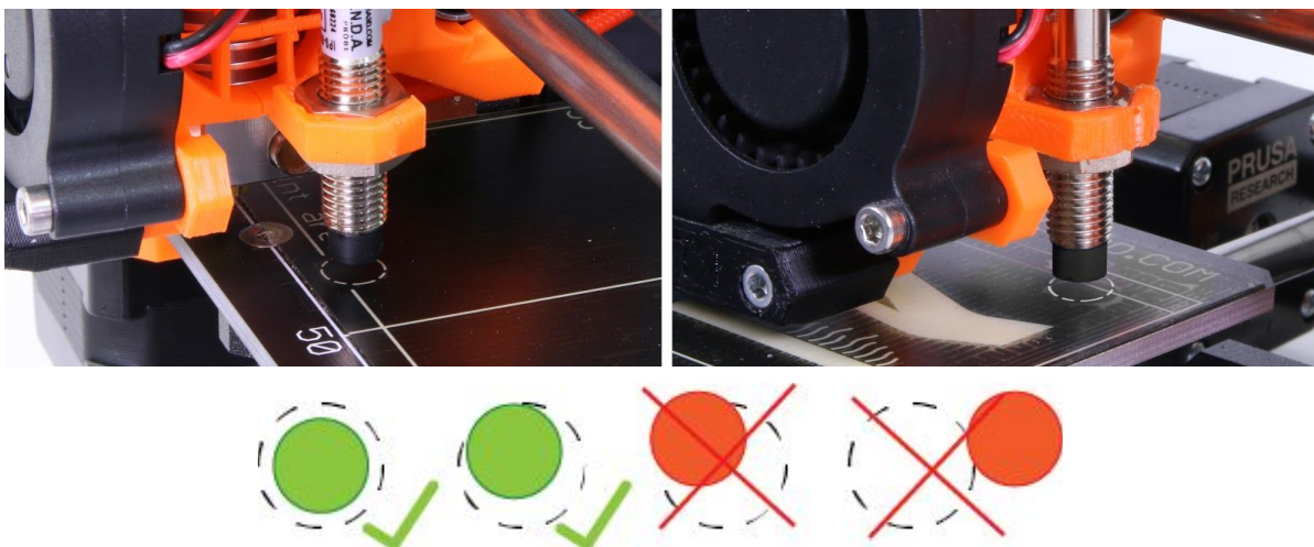
Pic. 6 - The probe must be inside the circles (1st and 9th calibration point) to successfully level the bed.
