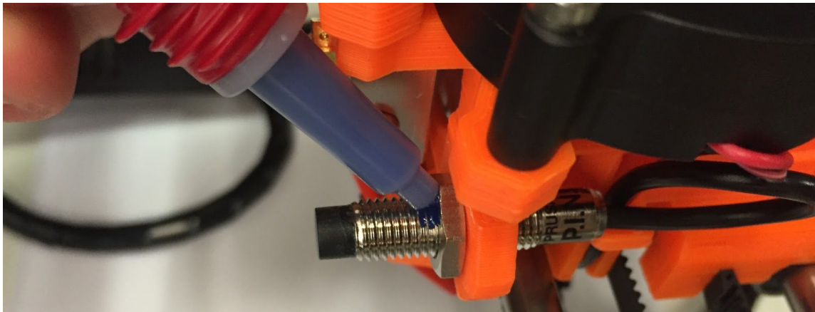
Pict. 12 - Secure the bottom nut on the probe with a drop of Loctite 243
