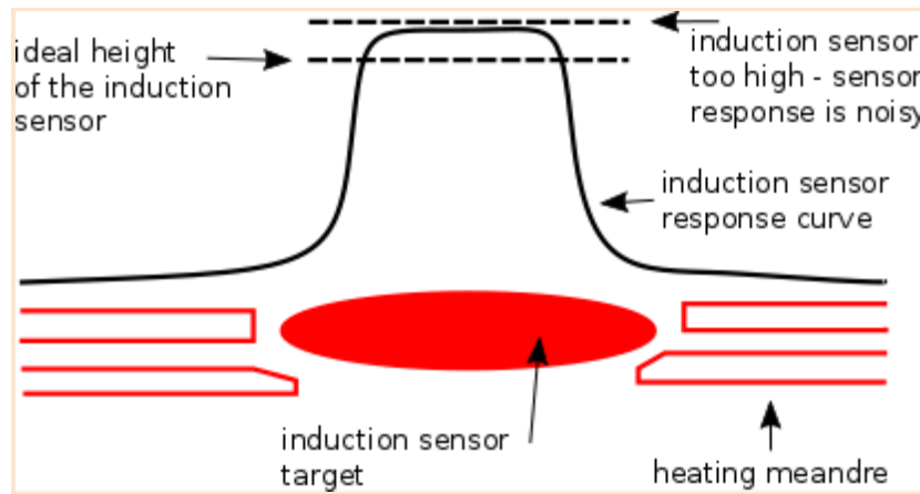
Pic. 11 - Probe response diagram.
